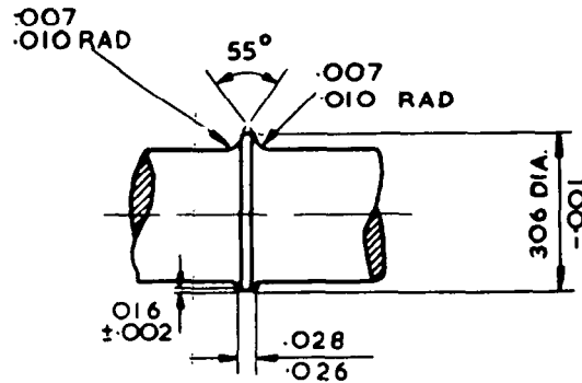
DETAIL AT Z'
