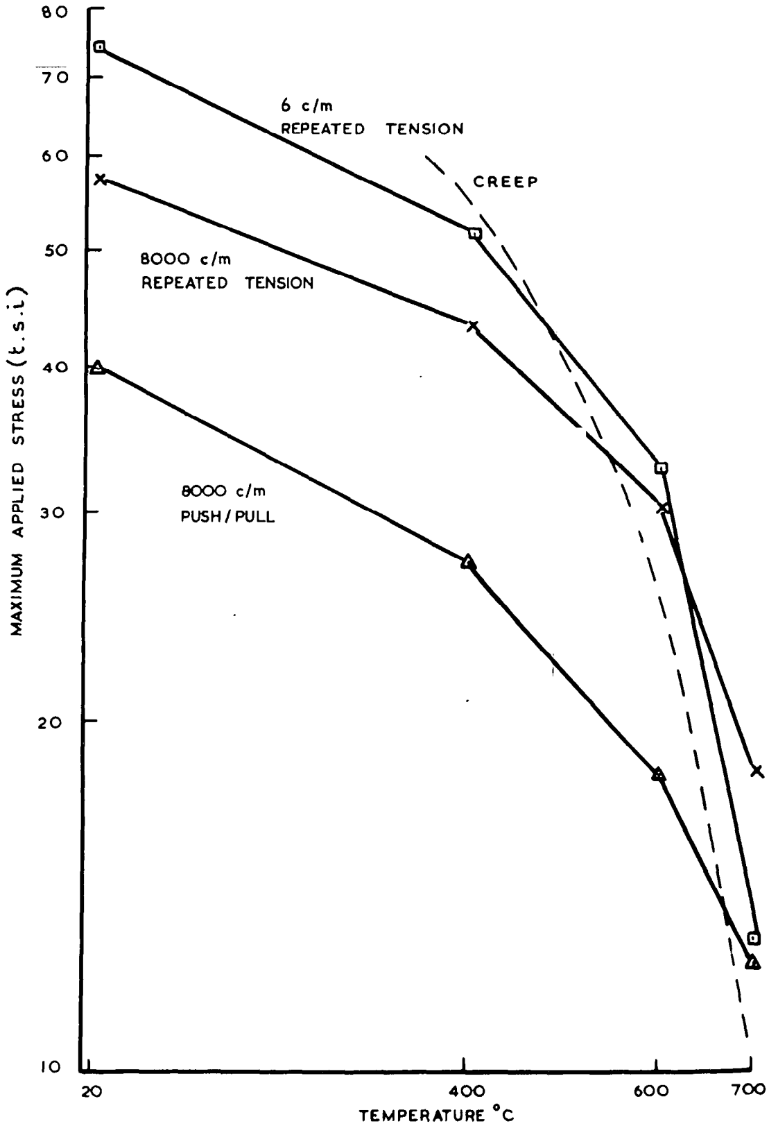
STRESS/TEMPERATURE FATIGUE & CREEP 10HR. CROSS-PLOTS
