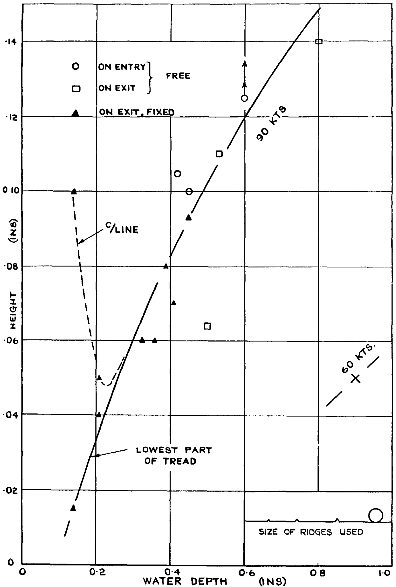
FIG.1. "AQUAPLANING HEIGHT" OF METEOR TYRE FROM RUNWAY, AT 90 KNOTS (RIBBED, 2 TON LOAD)
