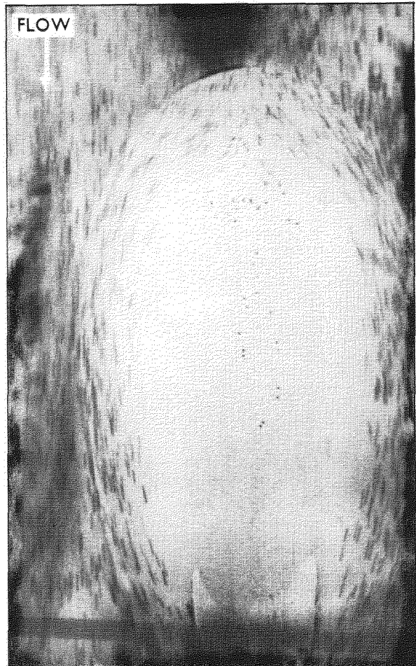
FIG.8. LOCKED 30 ft/sec., 1/16th in.
