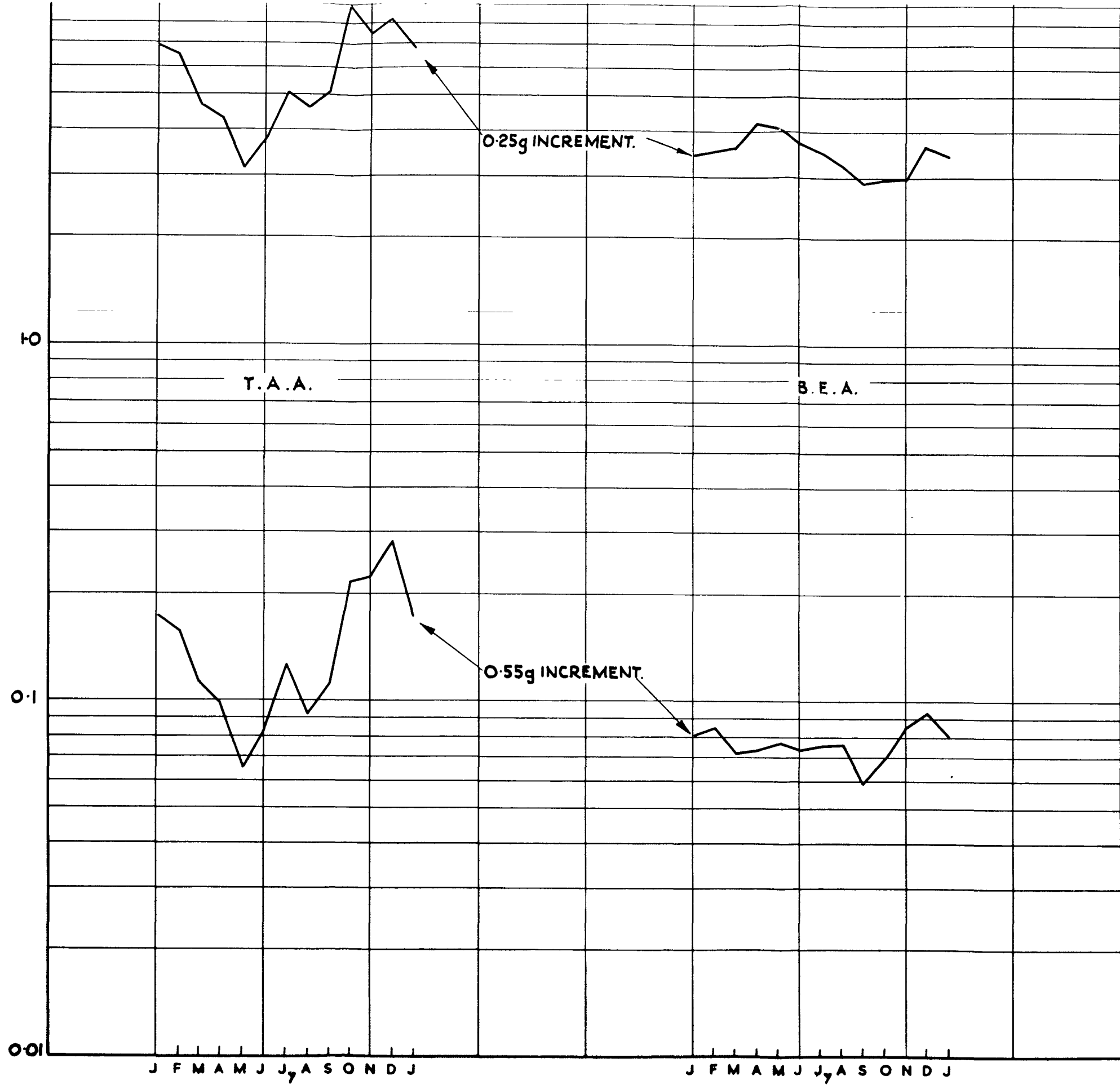
FIG. 4. COUNTS PER HOUR SUMMED OVER ALL AIRCRAFT, ALL YEARS, AT 0.25g AND 0.55g INCREMENT LEVELS - B.E.A. AND T.A.A. VISCOUNTS.
