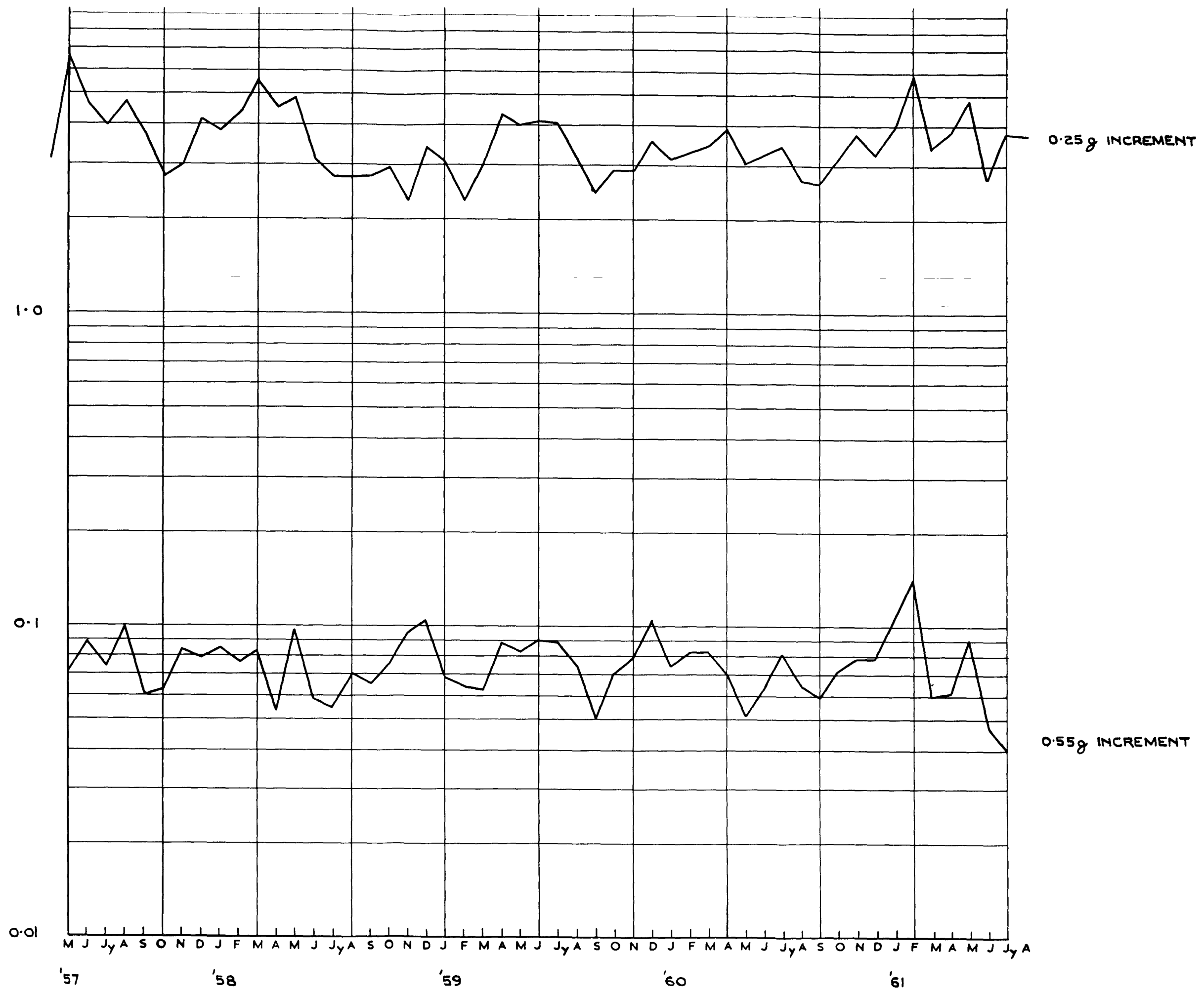
FIG. 2(a) COUNTS PER HOUR SUMMED OVER ALL AIRCRAFT, SUCCESSIVE YEARS, AT 0.25g AND 0.55g INCREMENT LEVELS—B.E.A. VISCOUNTS.
