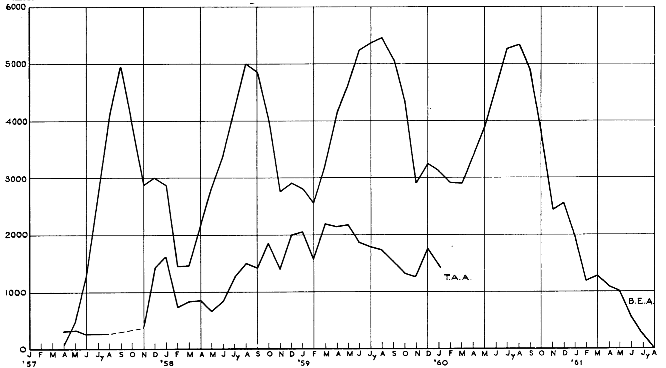
FIG.5. AIRCRAFT HOURS PER MONTH SUMMED OVER ALL AIRCRAFT, SUCCESSIVE YEARS - B.E.A. AND T.A.A. VISCOUNTS.
