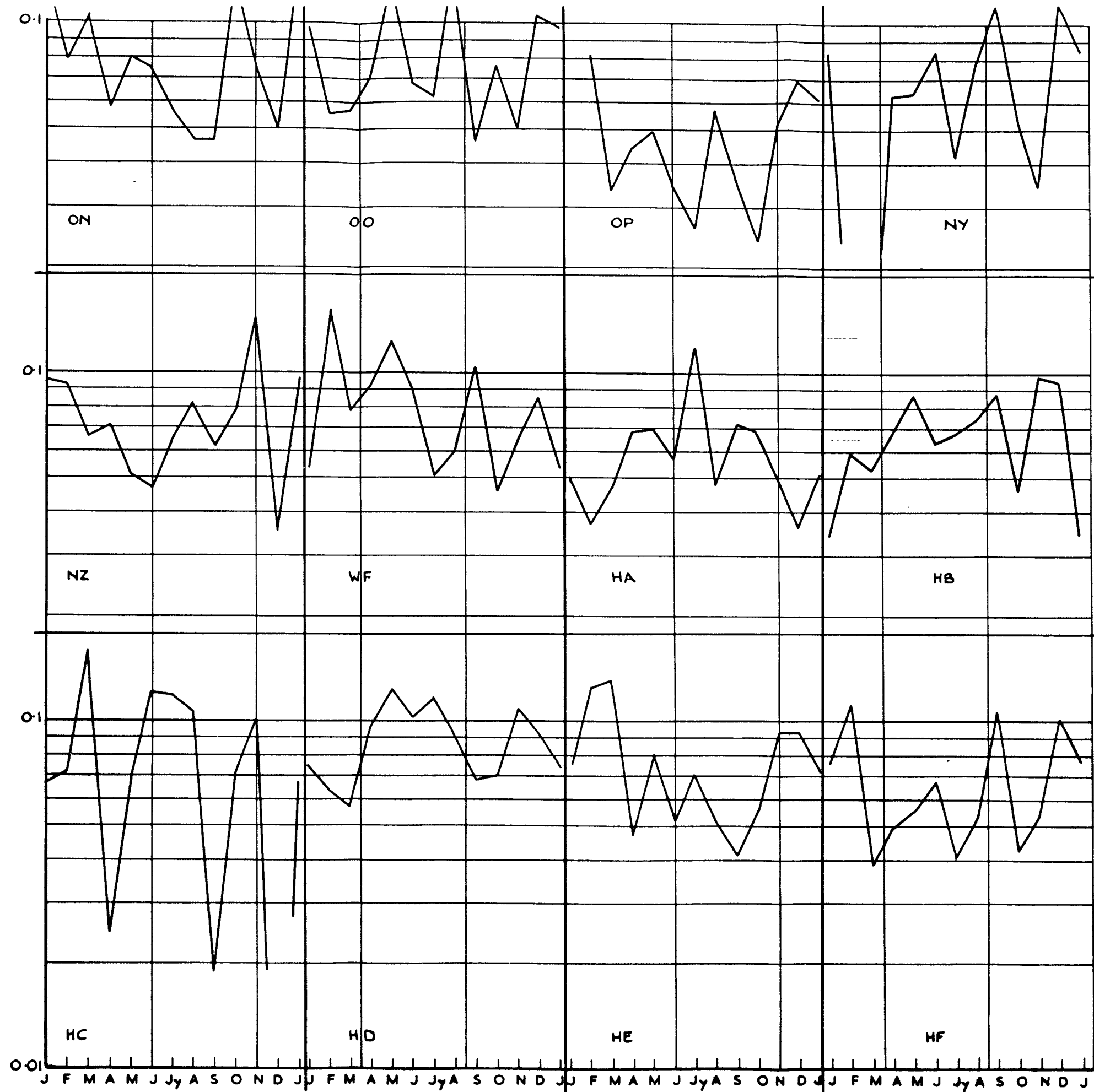
FIG.3 (e) COUNTS PER HOUR FOR INDIVIDUAL AIRCRAFT, SUMMED OVER ALL YEARS, AT 0.55a INCREMENT LEVEL - B.E.A. VISCOUNTS.
