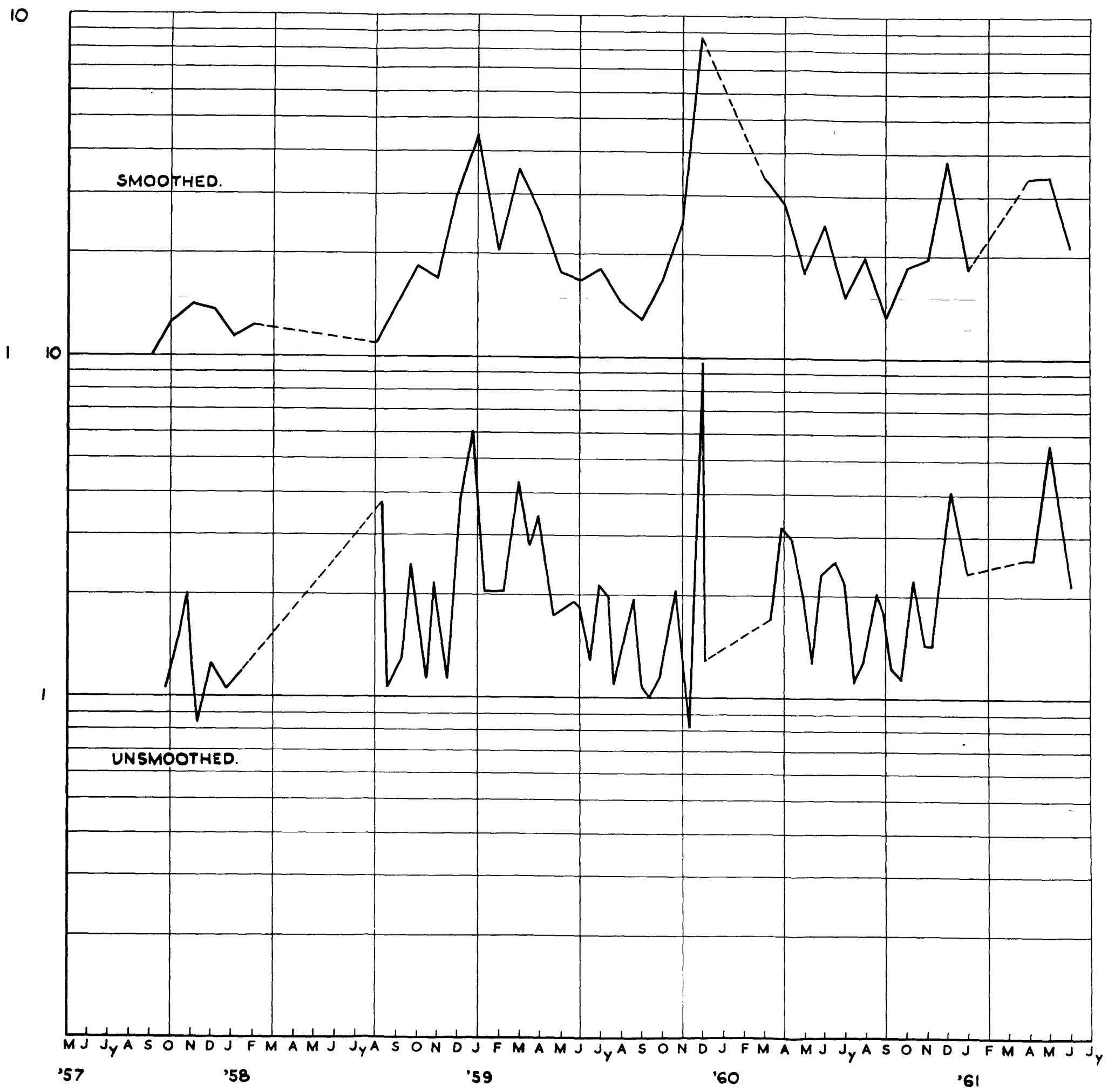
FIG. I. SMOOTHED AND UNSMOOTHED COUNTS PER HOUR FOR R.F.A. VISCOUNTS G-AMOI AT +0.25a INCREMENT LEVEL.
