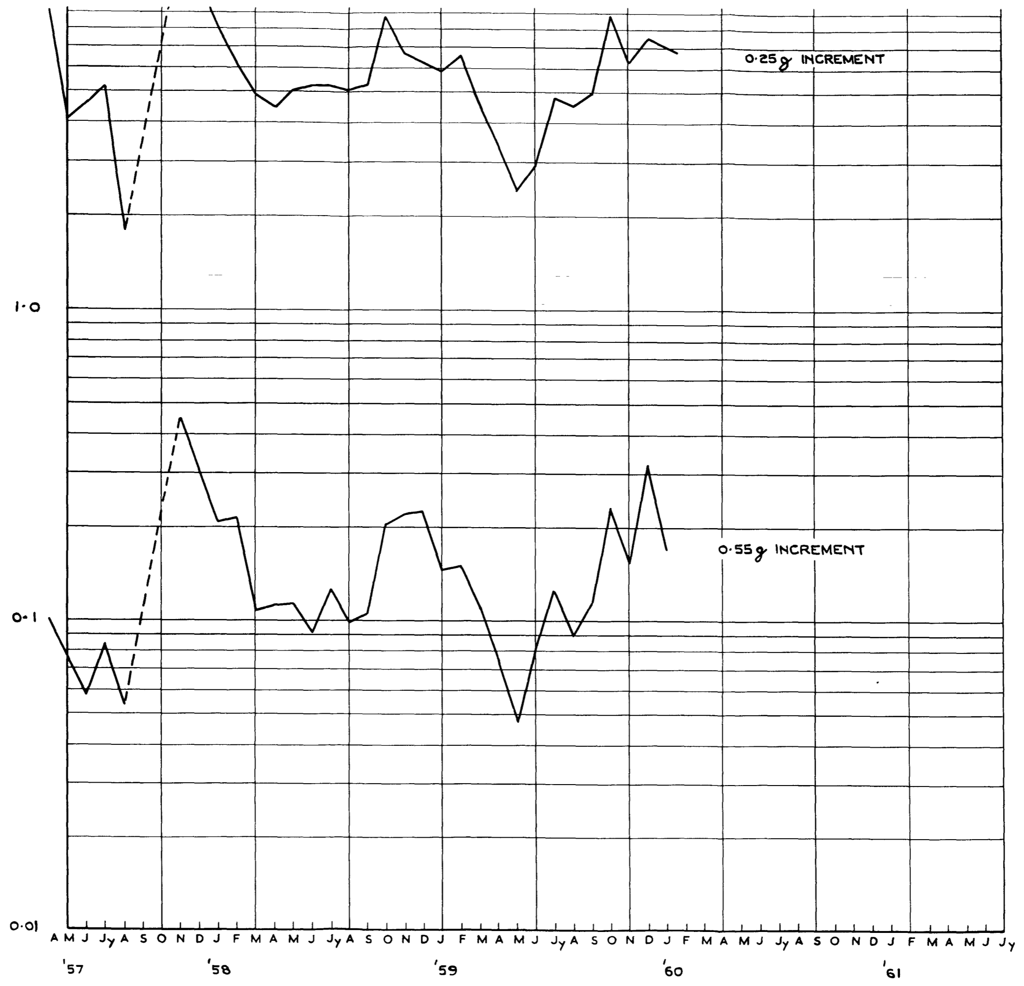
FIG. 2.(b) COUNTS PER HOUR SUMMED OVER ALL AIRCRAFT, SUCCESSIVE YEARS, AT 0.25g AND 0.55g INCREMENT LEVELS - T.A.A. VISCOUNTS.
