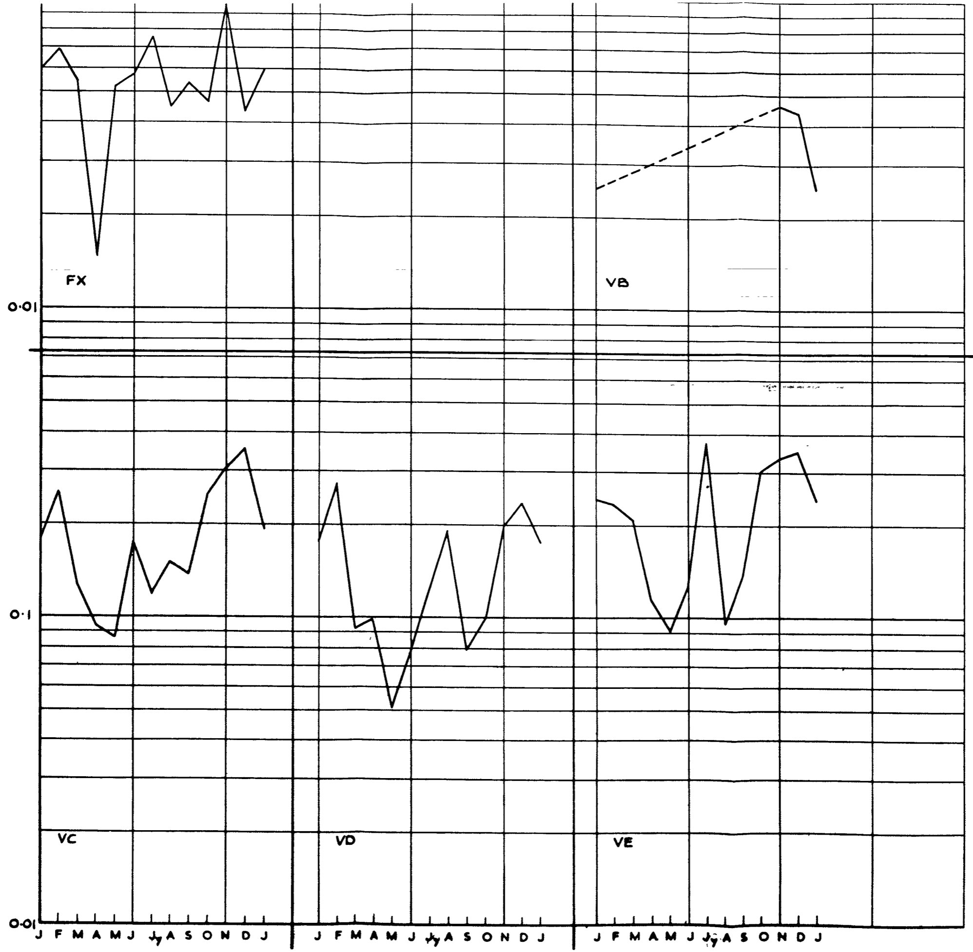
FIG. 3 (f) COUNTS PER HOUR FOR INDIVIDUAL AIRCRAFT, SUMMED OVER ALL YEARS, AT 0.55g INCREMENT LEVELS - B.E.A. AND T.A.A. VISCOUNTS.
