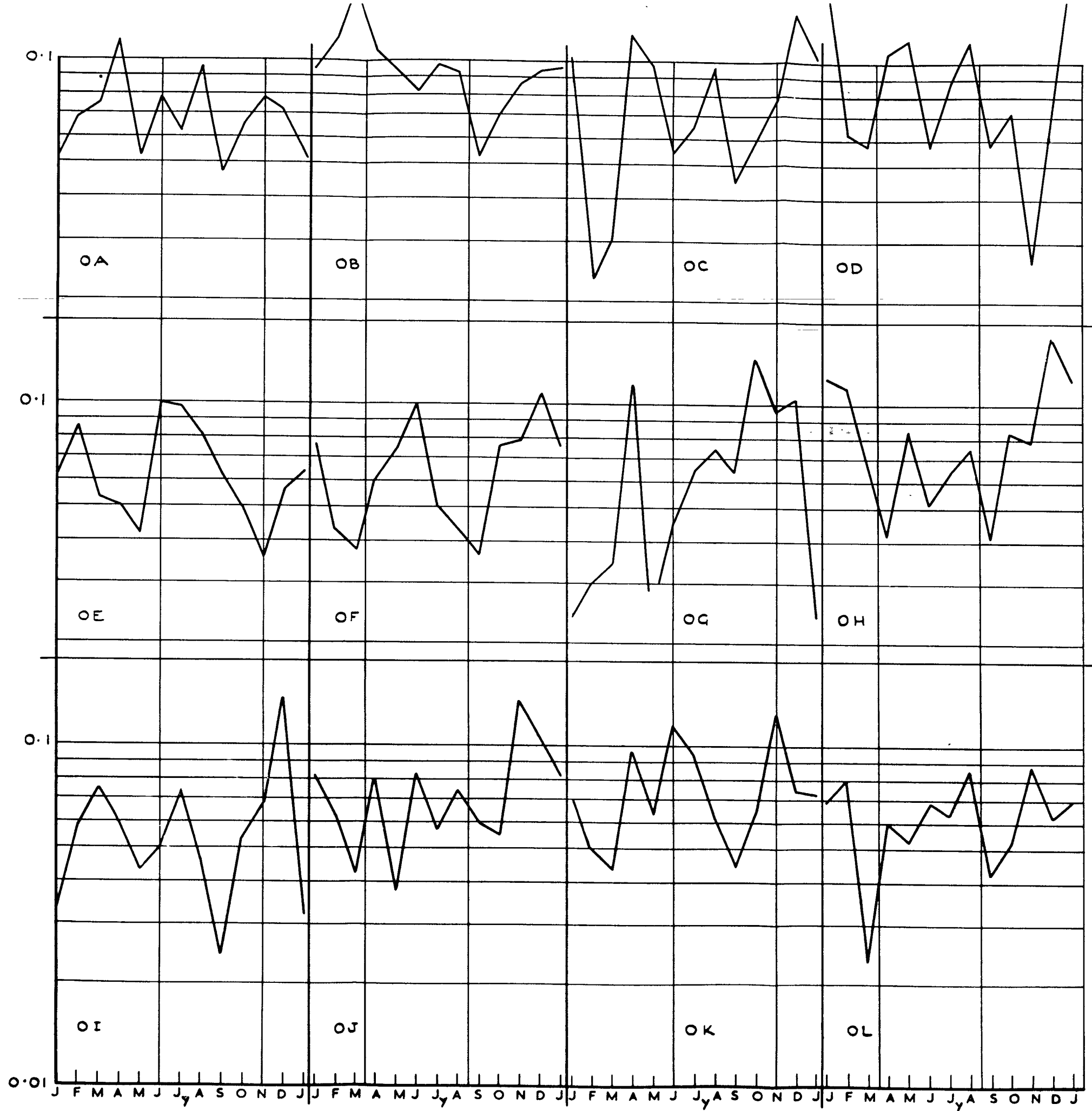
FIG.3.(d) COUNTS PER HOUR FOR INDIVIDUAL AIRCRAFT, SUMMED OVER ALL YEARS, AT 0.55g INCREMENT LEVEL - B.E.A. VISCOUNTS.
