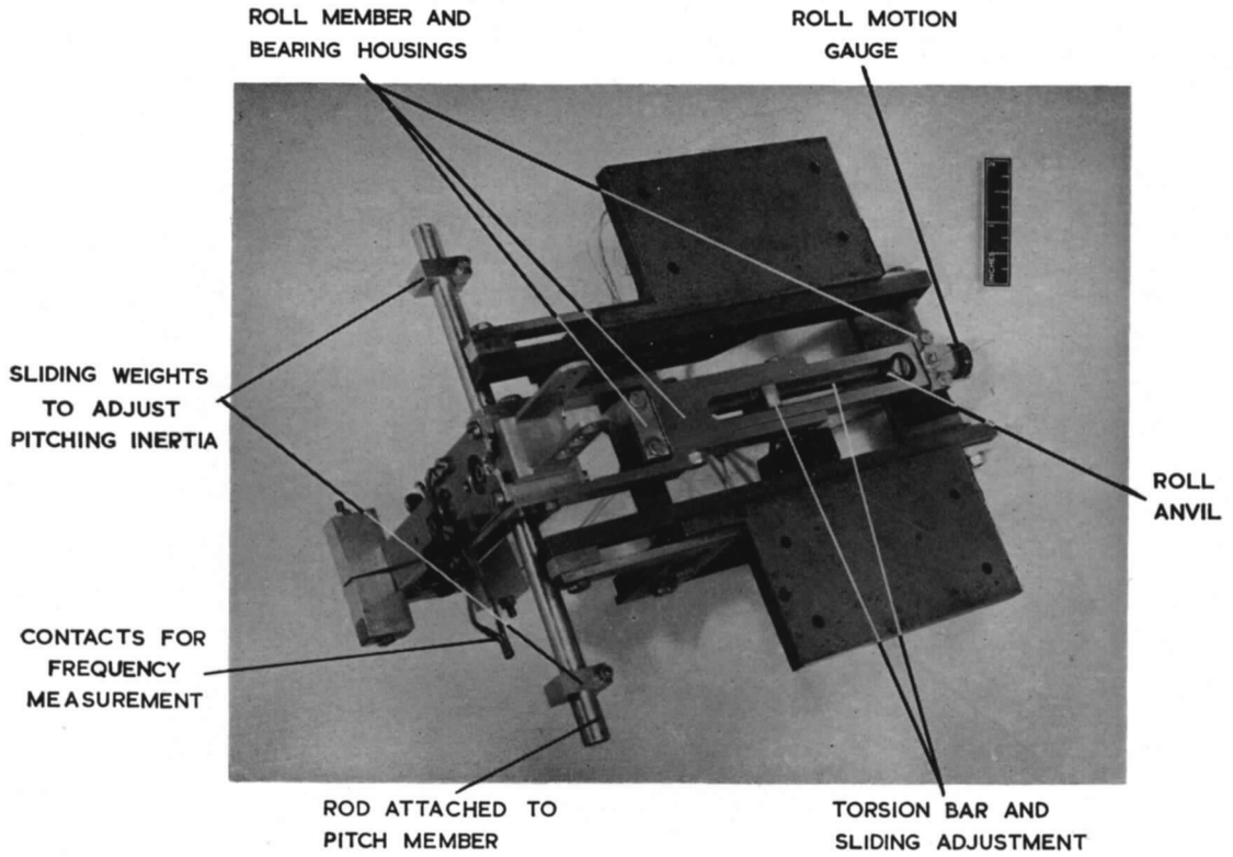
FIG. 1. Plan view.
