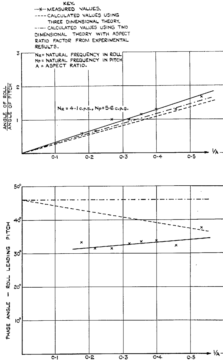
FIG. 4. The effect of aspect ratio on amplitude ratio and phase angle.
