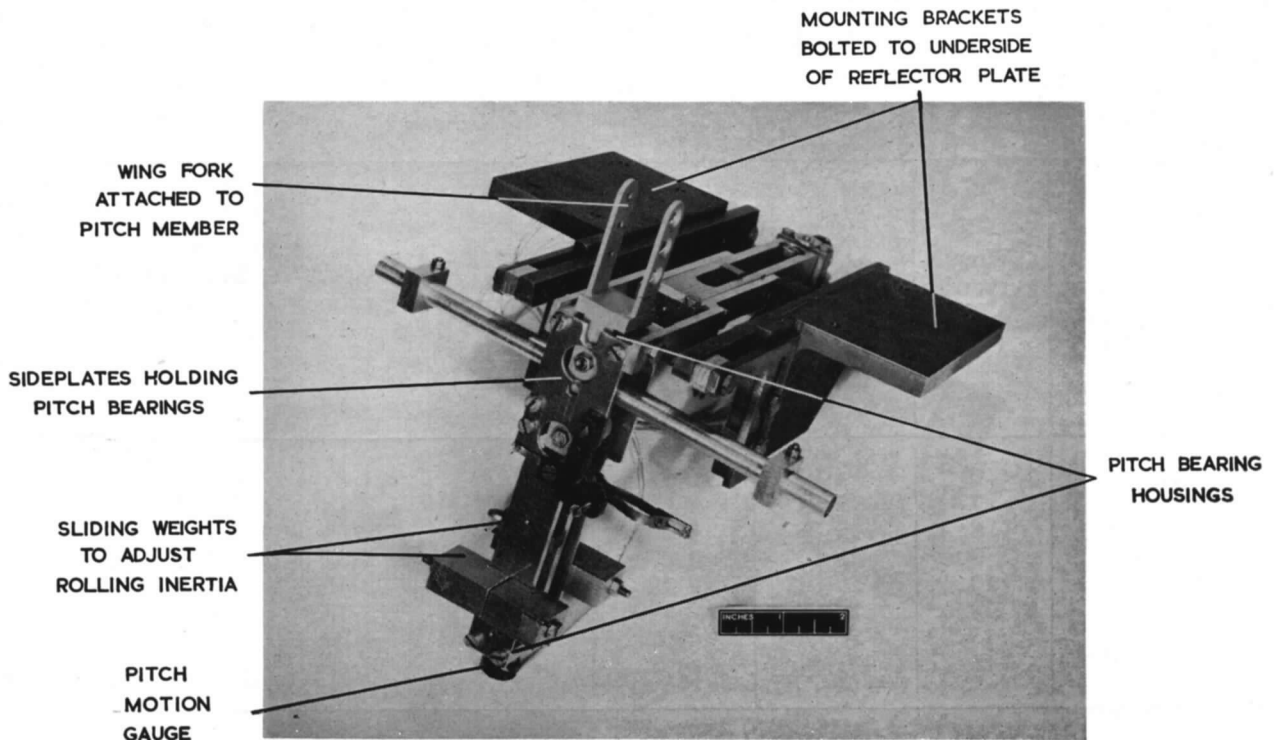
FIG. 2. Front elevation.
