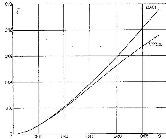
FIG. 17. Maximum supercelocity ratio for ellipsoids of varying thickness ratio, from exact and approximate methods.
