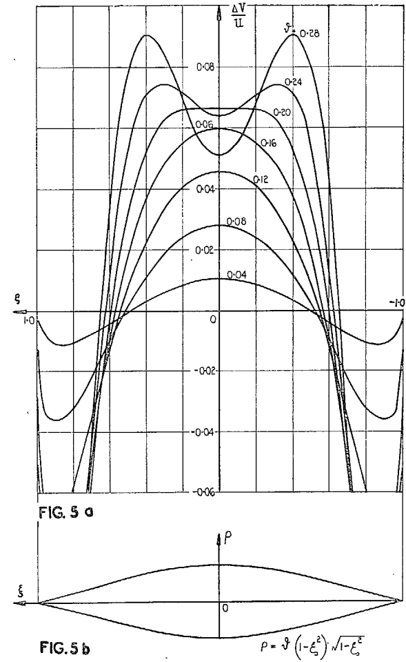
FIGS. 5, 5a and 5b. Induced velocity components and supervelocities for simple symmetrical bodies with cusped nose and tail end.
