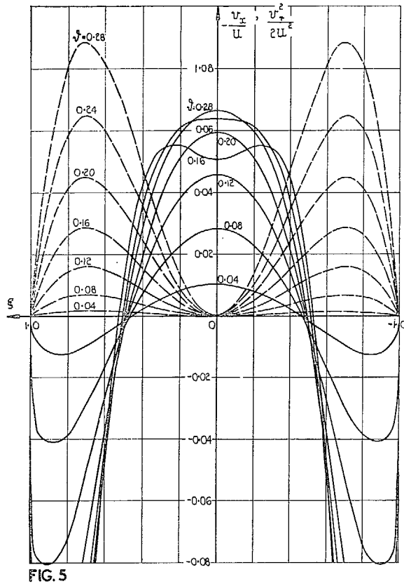
FIGS. 5, 5a and 5b. Induced velocity components and supervelocities for simple symmetrical bodies with cusped nose and tail end.
