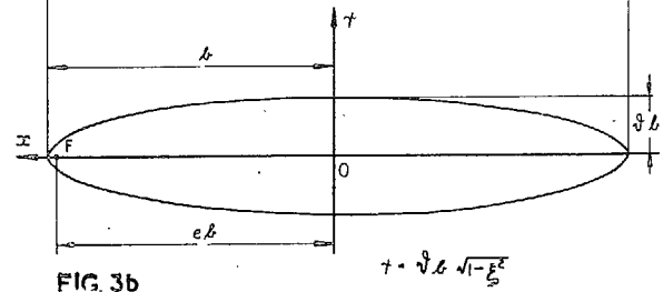
Figs. 3, 3a and 3b. Induced velocity components and resultant supervelocities for elongated ellipsoids of revolution.
