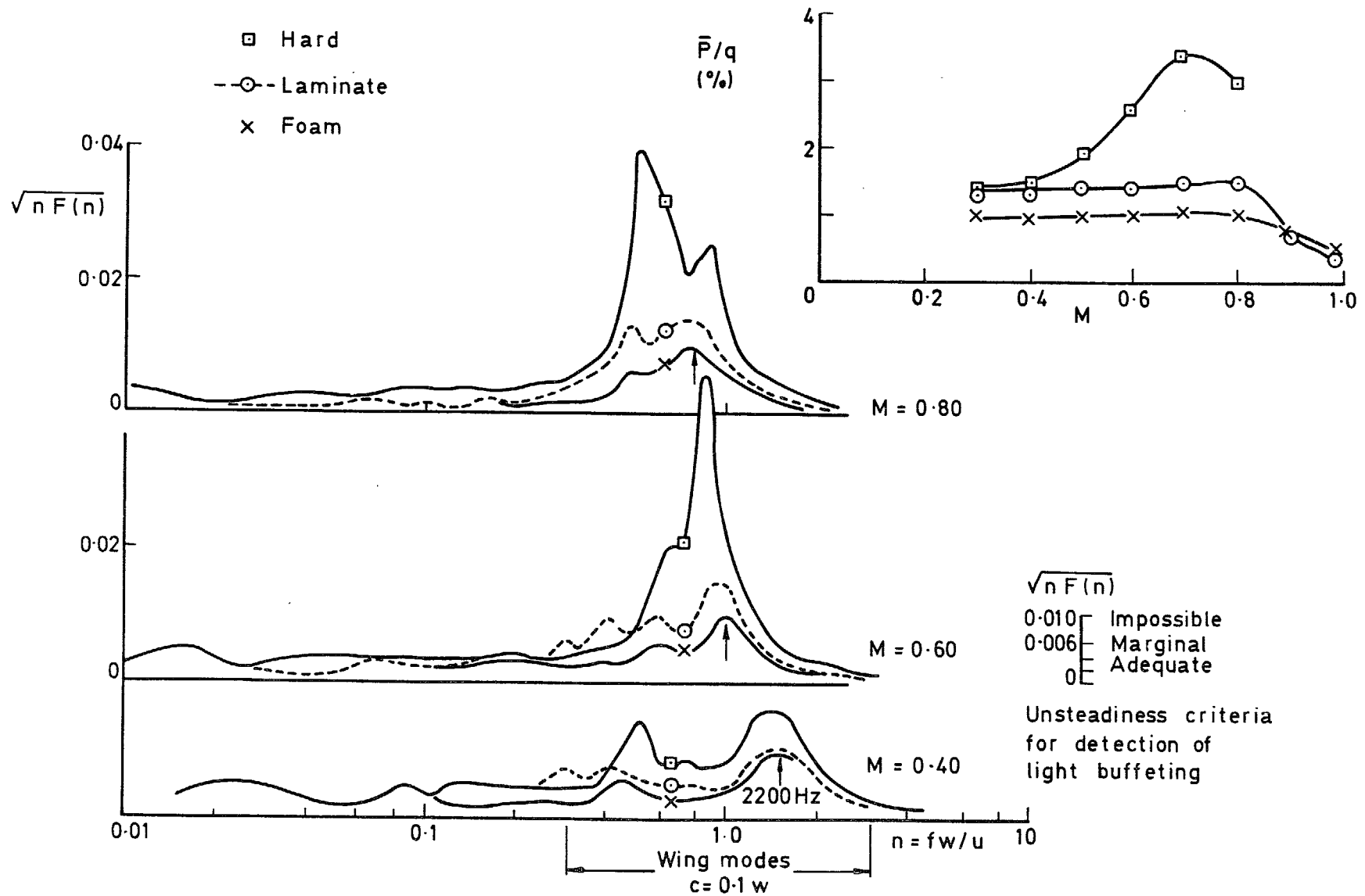
Fig 23 4in x 4in slotted working sections – pressure fluctuations at X/H = 2.5 tunnel empty
