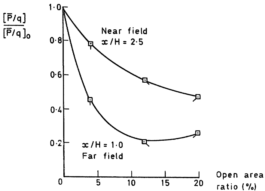
b Attenuation of pressure fluctuations with open area ratio
