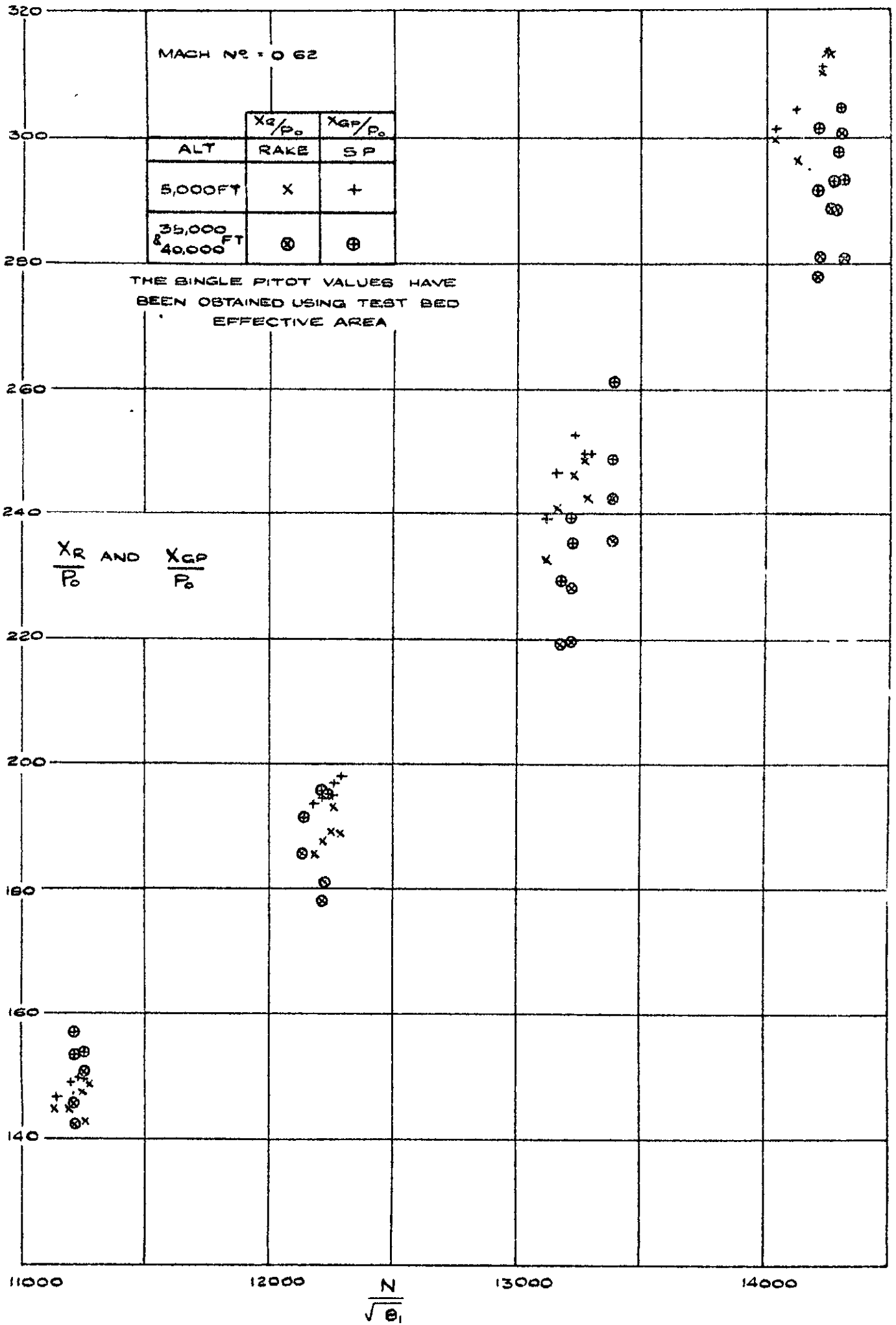
FLIGHT THRUST MEASURED BY RAKE \frac{X_R}{P_0} AND BY SINGLE PITOT \frac{X_{GP}}{P_0} AT 5,000 FT. AND 35,000 FT AT MACH. N° = 0.62 PLOTTED AGAINST \frac{N}{\sqrt{e_1}}
