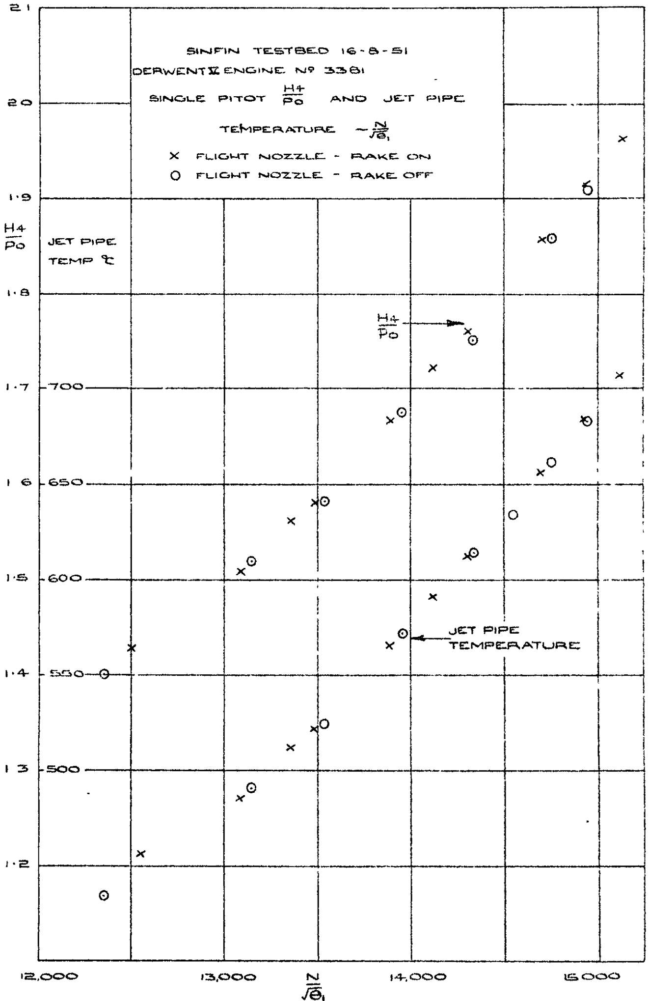
EFFECT OF PRESENCE OF PITOT RAKE ON JET PIPE TEMPERATURE & SINGLE PITOT. TEST BED RESULTS.
