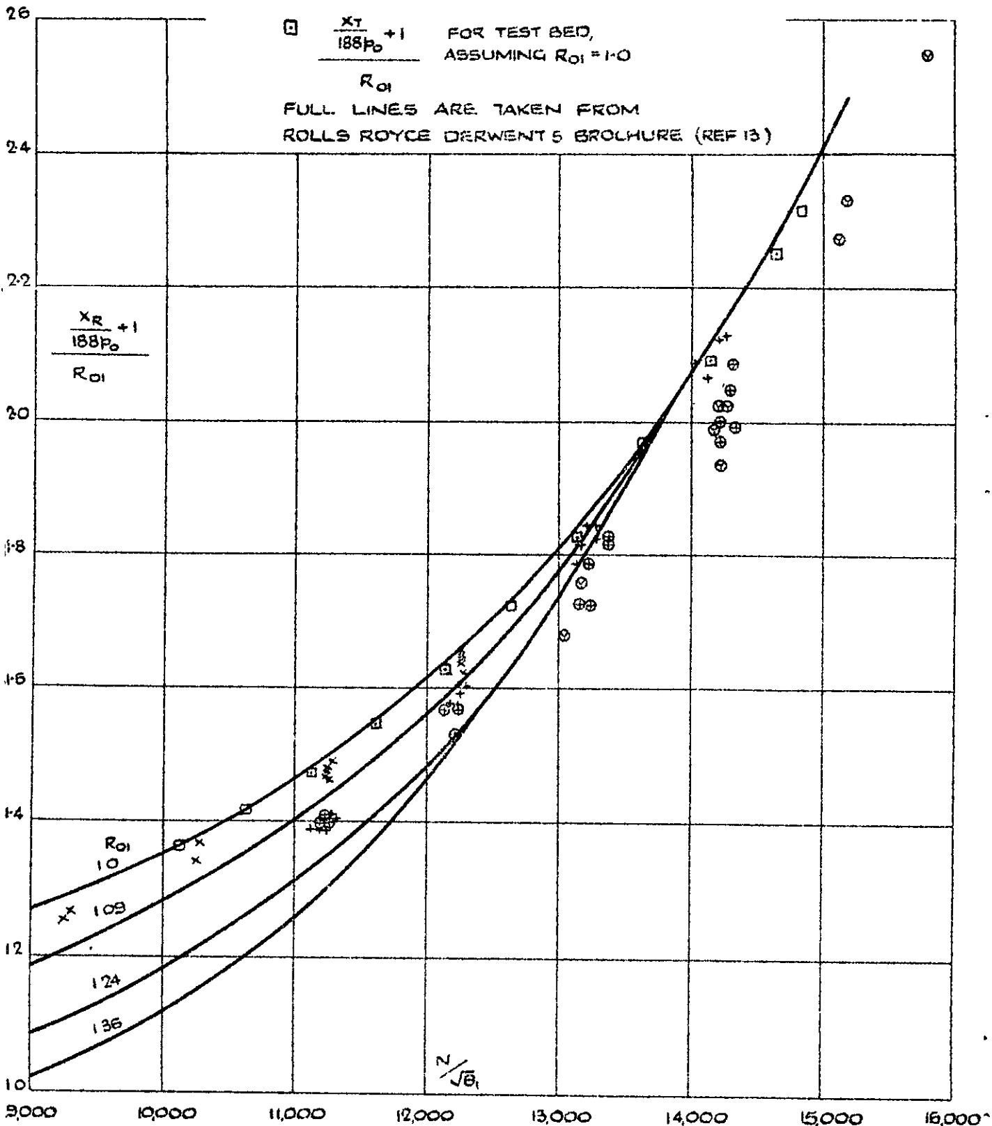
PLOT OF \frac{X_R}{188P_0} + 1 AGAINST \frac{N}{\sqrt{W}} FOR FLIGHT MEASUREMENTS, & COMPARISON WITH TEST BED, THRUSTMETER AND BROCHURE FIGURES.
