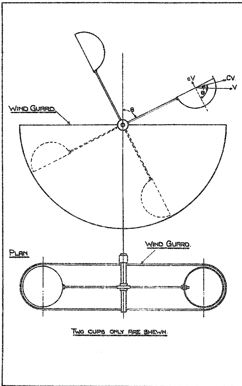
DIAGRAM OF THE HEMISPHERICAL CUP.
