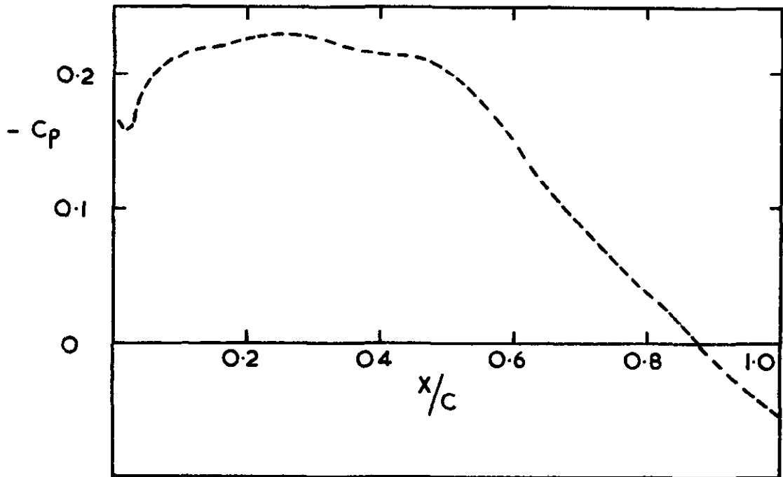
Fig.3 Measured pressure distribution on 55^\circ swept wing model at M = 0.55 , \alpha = 2^\circ , R_c = 27 \times 10^6
