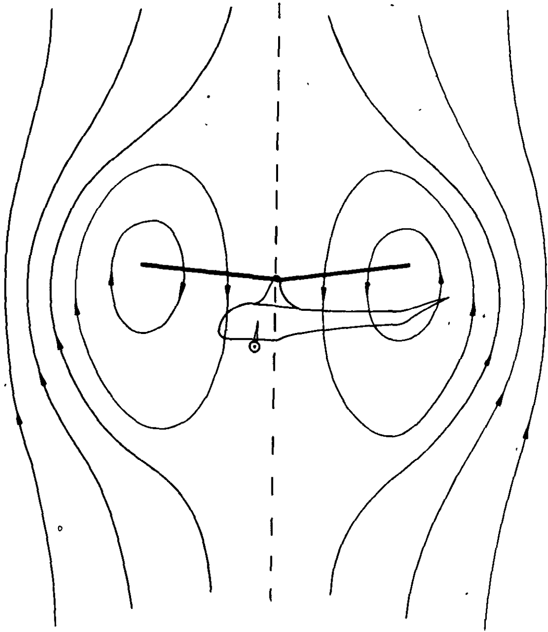
FIG.2. TYPICAL VORTEX RING FLOW PATTERN.
